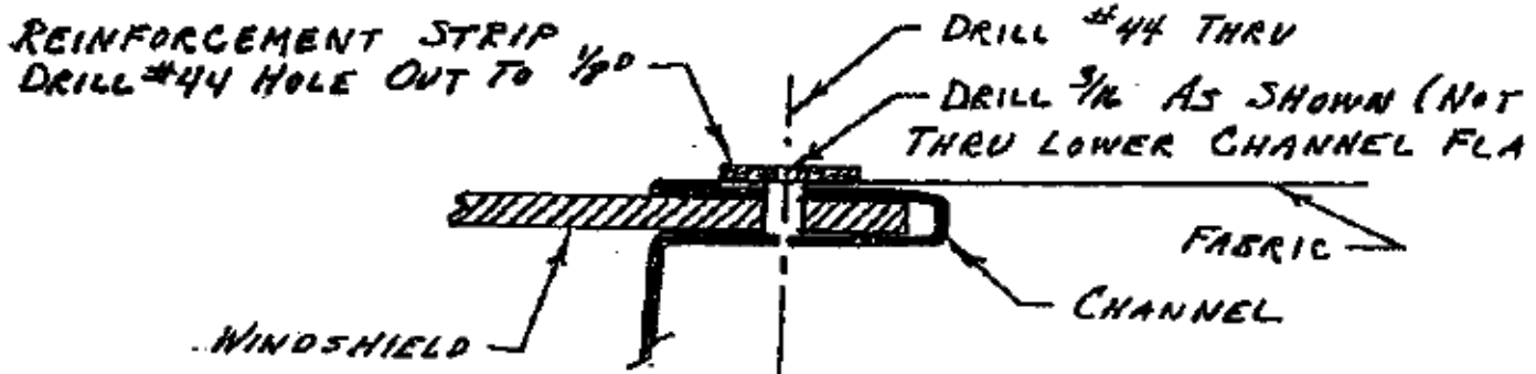
DETAIL DRILLING OF SCREW HOLES.
